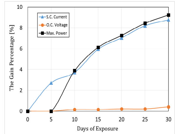
Fig. 7. Second test results, gain percentage of the short circuit current, open circuit voltage and maximum power along the test period
