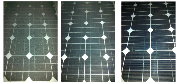
Fig. 8. Photographs of the tested PV module After 30 days, from left to right uncovered, covered and cleaned module respectively
