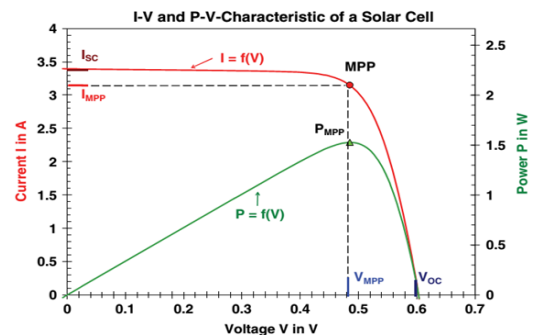
Fig. 4. Characteristic curves I-V and P-V of a typical mono-crystalline silicon solar cell
