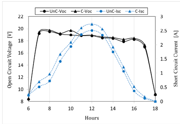
Fig. 5. First test results, hourly measured open circuit voltage and short circuit current for 1 st October
