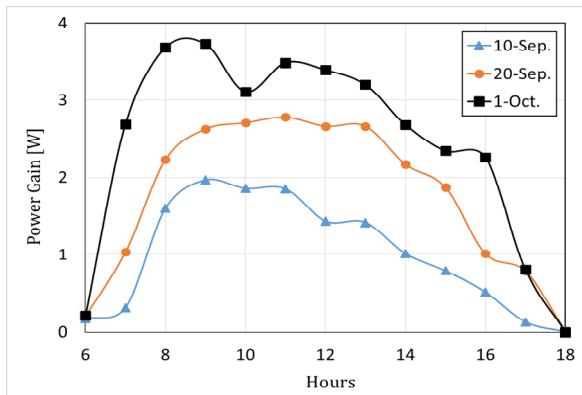
Fig. 6. First test results, hourly power gain for three dates
